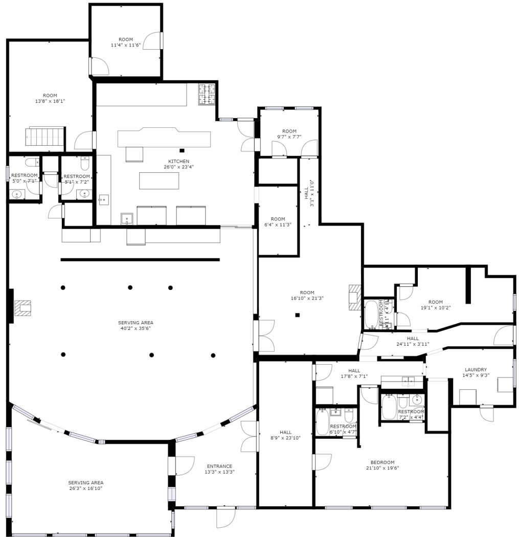
FLOOR 2
